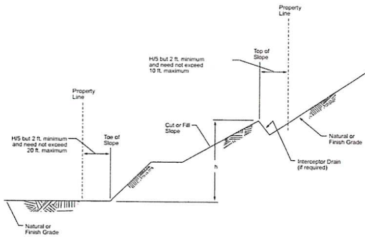
Figure 3.9.2 Setbacks
