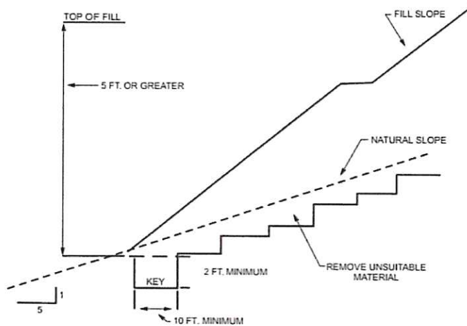
Figure 3.9.1 Benching Details
